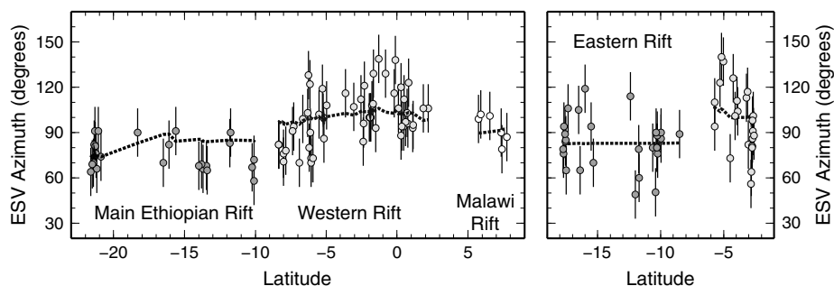
Figure 4. Comparison between observed earthquake slip vector directions (circles) and prediction of the best fit model along the different segments of the East African Rift. Error bars are 95% confidence.
