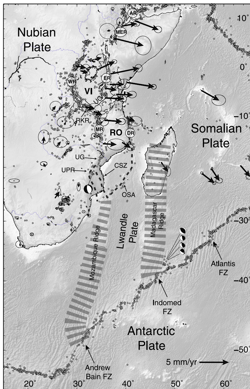
Figure 1. Present-day tectonic setting of the East African Rift. Solid black lines show major active faults [from Skobelev et al. , 2004], small black circles show seismicity (National Earthquake Information Center (NEIC) catalog), dashed lines indicate inferred plate boundary traces, and hatched areas over Madagascar and the Madagascar Ridge show the possibly diffuse Lwandle-Somalia plate boundary. Black arrows show a selection of the GPS data set used here, with 95% confidence ellipses. The focal mechanism of the M_{7.5} , 22 February 2006, Mozambique earthquake is shown [Fenton and Bommer, 2006], as well as the focal mechanisms of a cluster of thrust events at the southern end of the Madagascar Ridge (NEIC). MER = Main Ethiopian Rift, WR = Western Rift, ER = Eastern Rift, MR = Malawi Rift, DR = Davie Ridge, CSZ = Chissenga seismic zone, UG = Urema graben, UPR = Urrongas protorift, USA = Quathlamba Seismic Axis, RK = Rukwa, and UG = Usangu basin.
