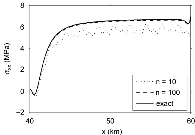
Fig. 9. Stresses from a triangular dislocation element and variable resolution rectangular approximations. Triangle lies in y – z plane with a width and depth of 20 km. Stresses are calculated along a set of observation coordinates parallel to dipping leg of a triangular dislocation element and offset in y direction by 1 km. Triangle surface is approximated using multiple rectangular dislocations whose edges match exactly except along bottom dipping leg of triangle. Stresses from rectangular approximations of triangular dislocation converge as the number of rectangular elements increases.
