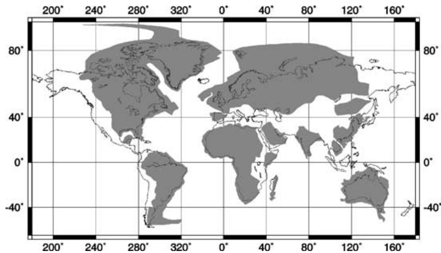
Figure 1. Stable continental regions (SCRs: light grey). We consider seven large SCR in this study: North America, South America, Eurasia (subdivided into Europe, west of 20°E, and Russia, east of 20°E), Africa (including the Arabian peninsula), India, China (consisting of three separate SCR) and Australia. Antarctica is not included.
