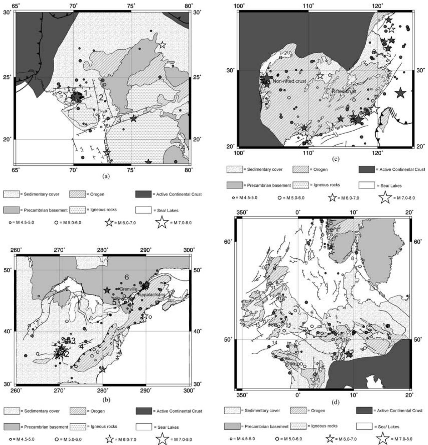
Figure 5. Simplified tectonic maps for different regions within stable continental crust and earthquakes from the database. Events that were recorded instrumentally are coloured dark grey, historic events are denoted by open symbols. (a) India, with (1) Kutch Rift, (2) Cambay rift, (3) Narmada Son rift and (4) Pranhita-Godavari rift. (b) Northeastern USA/Canada with (1) Midcontinent rift, (2) Reelfoot rift, (3) Rough Creek rift, (4) Rome trough, (5) St. Lawrence depression and (6) Ottawa rift. (c) Southern China, with East China rift system. (d) Europe with (1) Lower Rhine rift, (2) Upper Rhine rift, (3) Illies rift cluster, (4) Limange rift, (5) Brittany rift, (6) West Netherlands Sole Pit, (7) Central graben, (8) Oslo rift, (9) Viking graben, (10) Minches basin, (11) Midland valley, (12) Solway–Northumberland basin, (13) North Celtic sea basin, (14) Western Approaches basin and (15) Worcester basin.
