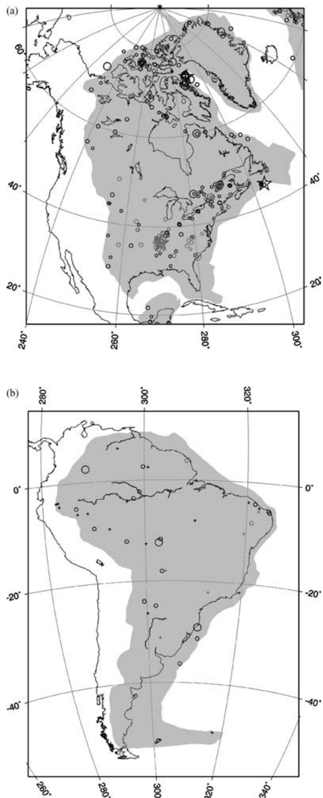
Figure 2. Earthquakes in the updated global database for the different stable continental regions (SCRs). Earthquakes with instrumentally determined location and magnitude are denoted by dark grey circles, historical events by light grey circles. (a) North America, (b) South America, (c) Europe, (d) Russia, India and China, (e) Africa, (f) Australia. Stars indicate M = 8 events. In b–e, crosses are smaller (4.5–5.0) events.
