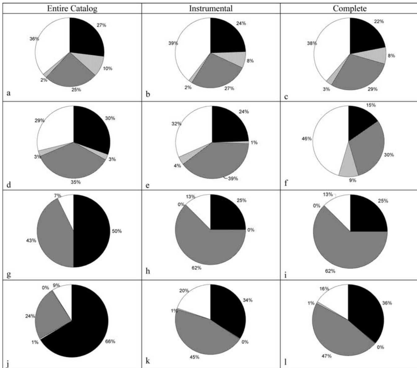
Figure 3. Distribution of seismicity over the five different categories for entire database of instrumentally recorded events and complete subset events: rifts (black), possible rifts (stippled), rifted margins (striped), possible rifted margins (grey), non-rifted crust (white). (a)–(c) M \geq 4.5 events, (d)–(f) M \geq 6.0 , (g)–(i) M \geq 7.0 events and (j)–(l) seismic moment release.
