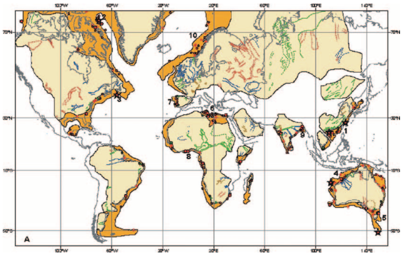
Figure 4. Earthquakes from the database for: (a) rifted continental margins; (b) interior rifts/taphrogens; and (c) non-extended continental crust. Extended margins are coloured orange, continental interiors yellow. Rifts and taphrogens are indicated with solid (boundaries are well determined) or dashed (boundaries are poorly determined) lines. Precambrian rifts are indicated in red, Palaeozoic in blue, Mesozoic in green and Cenozoic in brown. Maps were constructed from the Exxon tectonic maps (Exxon Production Research Company 1985) and the rift catalogue (Şengör & Natal' in 2001). Red circles denote events that are and green circles events that might possibly be associated with rifted continental margins or interior rifts, blue circles denote events that occur in non-rifted crust. Numbers indicate regions of concentrated seismicity and are those from Table 4.
