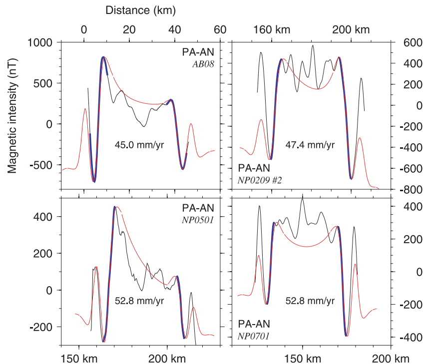
Figure 40. Cross-correlated fits of the Brunhes-Matuyama reversal for ridge-normal magnetic profiles from the sparsely surveyed Pacific–Antarctic rise west of 180^{\circ}\text{E} . Also see profile NP0209 #1 from Fig. 9. Black and blue lines show the observed profiles and red curves show the best-fitting synthetic magnetic profiles. The part of each observed profile that is cross-correlated with the synthetic profile is coloured blue. Profiles designated with the ‘NP’ identifier are unpublished transit tracks from the RV Nathaniel Palmer (S. Cande, personal communication, 2007).
