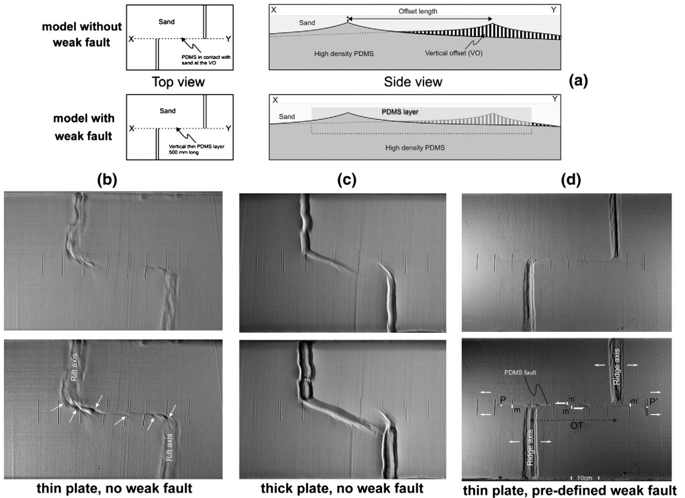
Fig. 6. Analog model with non-accreting brittle lithosphere by Marques et al. (2007). (a) Tested model setups. (b)–(d) Experimental results: (b) thin lithosphere at ridge axes, no embedded fault, (c) thick lithosphere at ridge axes, no embedded fault, (d) thin lithosphere at ridge axes, embedded weak fault.
