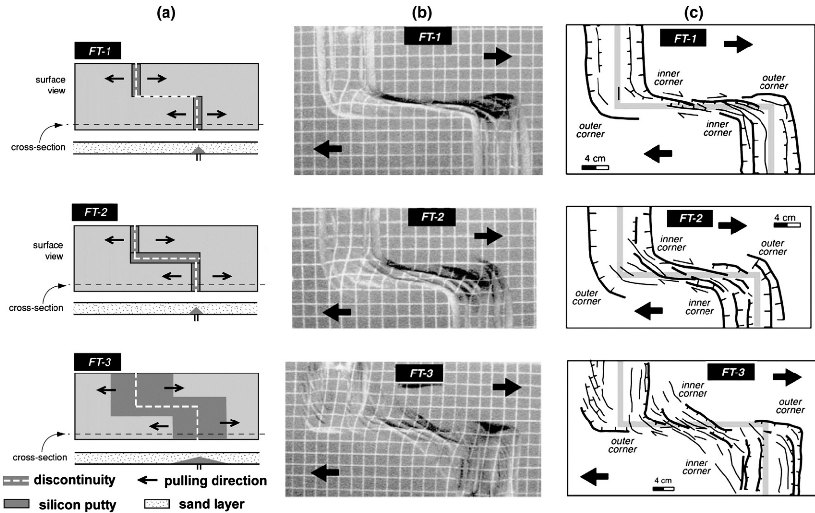
Fig. 5. Analog model with non-accreting brittle lithosphere by Dauteuil et al. (2002) . (a) Tested model setups: FT-1 without a silicone band on the transform discontinuity; FT-2 with a narrow silicone band on the transform discontinuity; FT-3 with a wide silicone band. (b), (c) Experimental results: (b) surface photographs of the experiments at the end of the deformation; (c) sketch drawings of fault patterns. The light gray line in (c) indicates initial location of diverging and transfer discontinuities.
