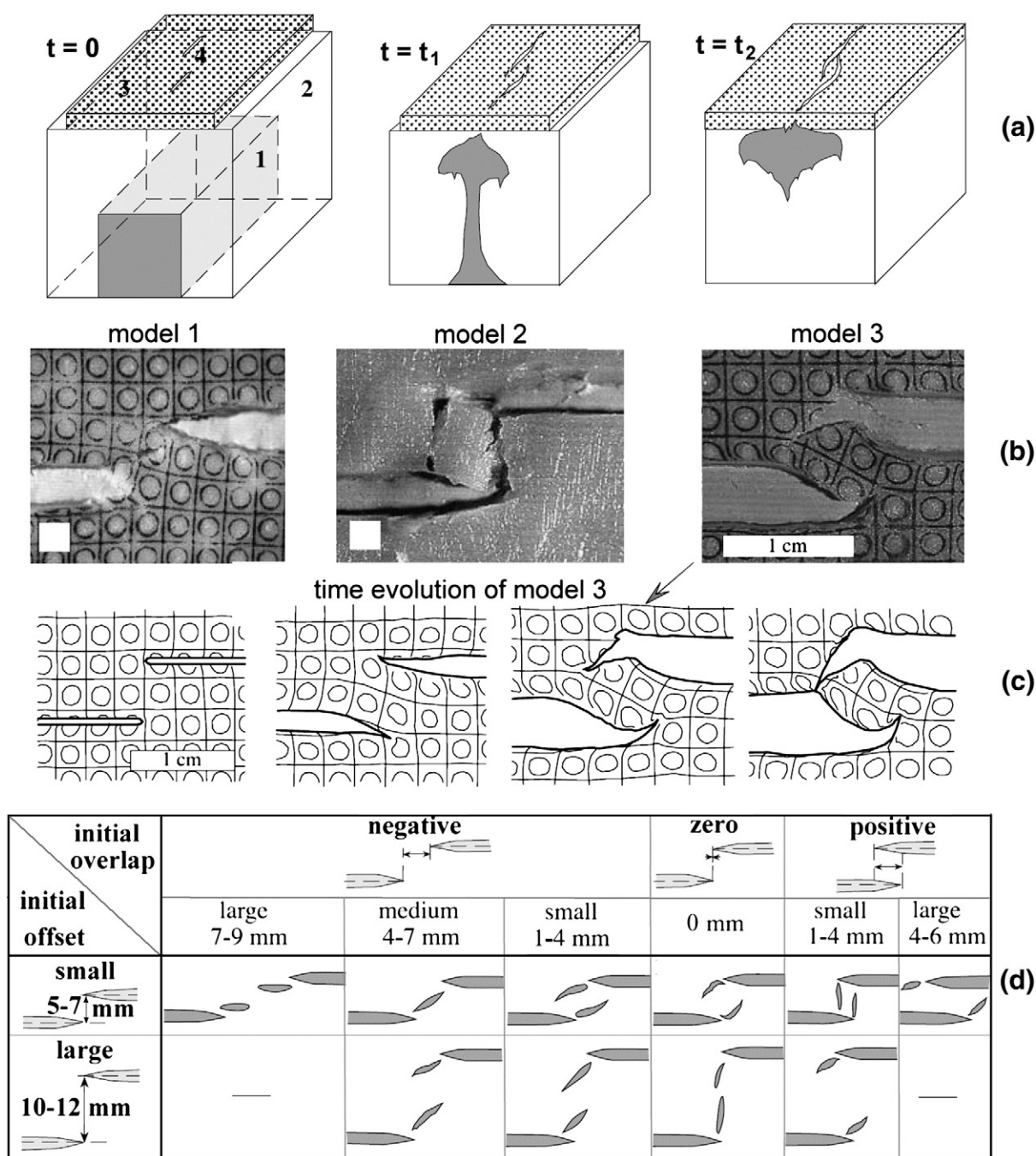
Fig. 7. Centrifuge model with non-accreting brittle lithosphere by Tentler and Aocella (2010). (a) Experimental setup: (1) lower-density silicone, simulating the asthenosphere; (2) higher-density silicone, simulating the upper mantle; (3) the uppermost brittle layer, simulating the oceanic lithosphere; and (4) precut fractures. (b) Examples of different types of fracture interactions in a map view. (c) Evolution of the reference model 3. (d) Types of interaction between two precut parallel fractures in the brittle layer of models.
