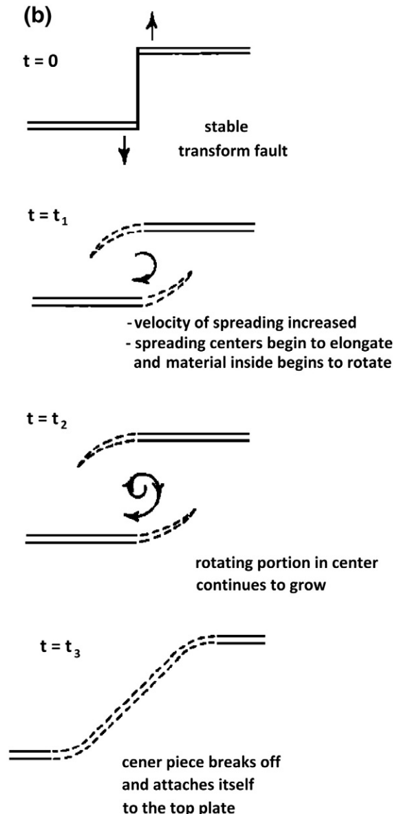
Fig. 2. Dynamics of formation (a) and destruction (b) of transform faults in freezing wax experiments (Oldenburg and Brune, 1975).
