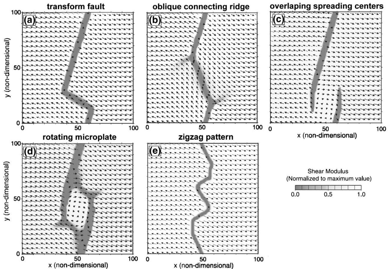
Fig. 9. Results of numerical experiments of Hieronymus (2004) showing fundamental modes of plate fragmentation with pre-defined ridge offset: (a) transform faults, (b) oblique connecting spreading centers, (c) overlapping spreading centers, (d) microplates, and (e) zigzag ridges.
