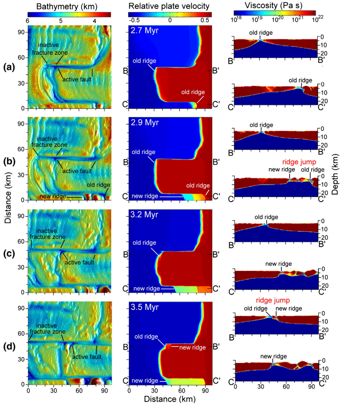
Fig. 12. Dynamics of development of inactive fracture zones after increase in the spreading rate (Gerya, 2010). Diagrams in (a)–(d) show successive stages of the process at 2.7, 2.9, 3.2 and 3.5 Myr, respectively: (a) stabilization of ridge offsets, nucleation of inactive fracture zones; (b)–(d) growth of inactive fracture zones, ridge jumps. Initial stages of model development correspond to Fig. 11a–c.
