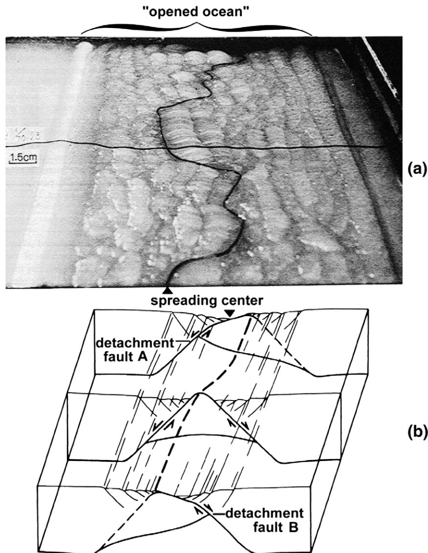
Fig. 4. Thermomechanical model of slow spreading by Shemenda and Grocholsky (1994): (a) model with strongly curved ridge, (b) schematic representation of transfer zone accommodating change in the polarity of spreading asymmetry to the opposite; two detachment faults (A and B) control the asymmetry.
