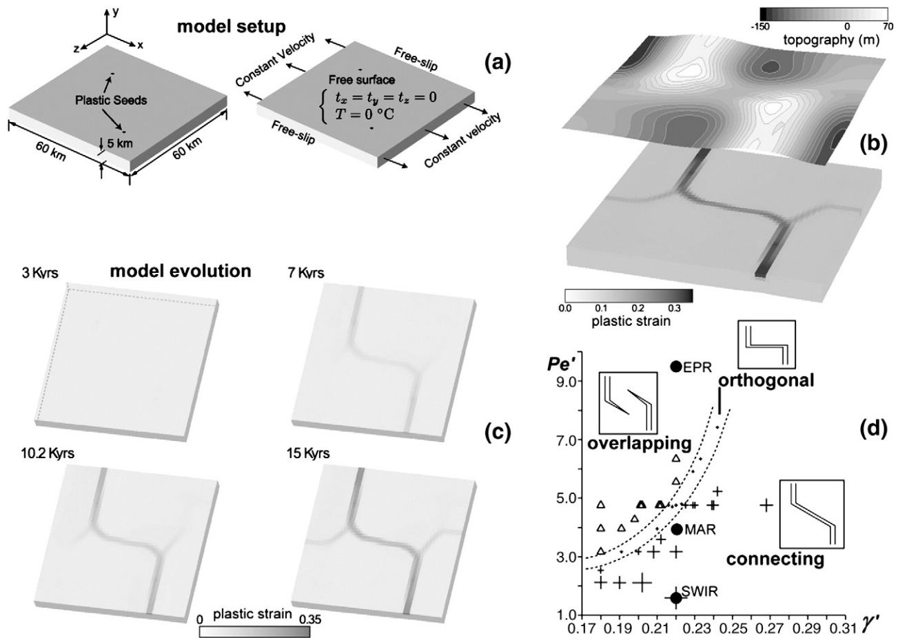
Fig. 10. 3D numerical experiments of Choi et al. (2008) on plate fragmentation with pre-existing ridge offset. (a) Model setup. (b) Model topography in case of an orthogonal ridge-transform fault pattern. (c) Development of the orthogonal pattern of plate fragmentation. (d) Summary of experimental results (symbols) and natural data (MAR = Mid Atlantic Ridge, EPR = East Pacific Rise, SWIR = Southwest Indian Ridge). Pe' is the spreading rate normalized by a reference cooling rate. \gamma' is the ratio of thermal stress to the reference spreading-induced stress.
