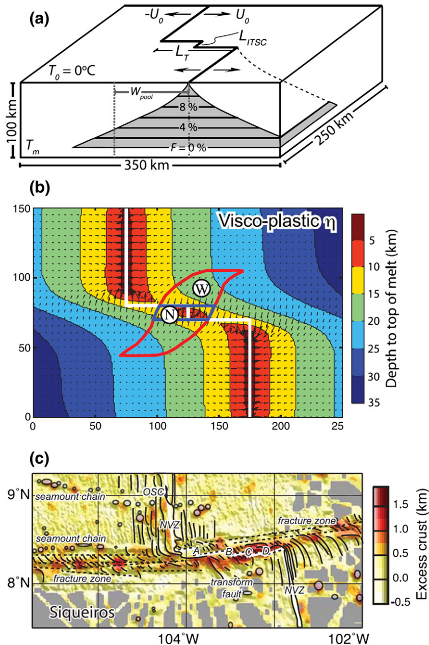
Fig. 8. 3D numerical modeling experiments of Gregg et al. (2009). (a) Model setup. (b) Calculated depth to the top of the melting region. Regions W (red outline) and N (blue outline) delineate the wide and the narrow melt pooling models, respectively. (c) Natural example of lateral variations in crustal thickness in transform fault derived from residual mantle Bouguer gravity calculations (Gregg et al., 2007). Excess crust is defined as the deviation for the reference crustal thickness of 6 km.
