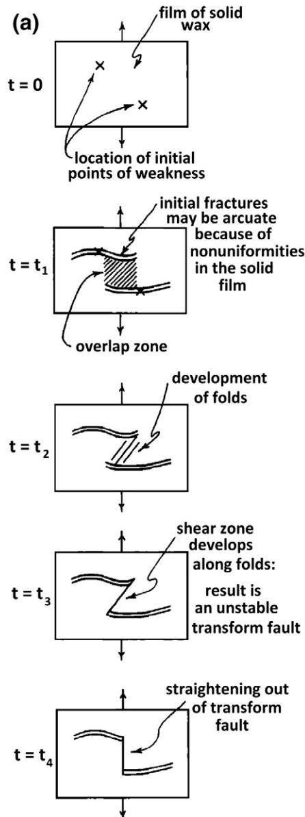
Fig. 2. Dynamics of formation (a) and destruction (b) of transform faults in freezing wax experiments (Oldenburg and Brune, 1975).
