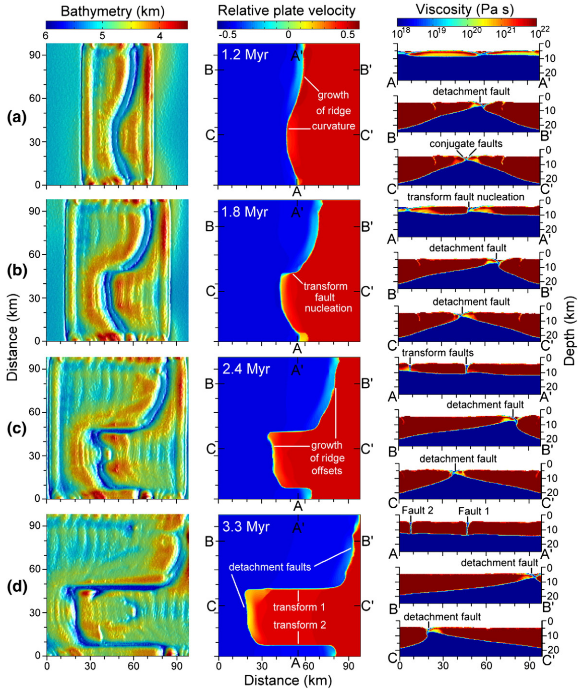
Fig. 11. 3D numerical experiments of Gerya (2010) showing spontaneous growth of transform faults at a single straight ridge. Sea level for bathymetry maps (left column) corresponds to the top of the model. Horizontal velocity in the middle column is normalized to the spreading rate. Diagrams in (a)–(d) show successive stages of the process at 1.2, 1.8, 2.4 and 3.3 Myr, respectively: (a) nucleation of ridge curvature; (b) nucleation of transform faults from the curved ridge sections; (c), (d) growth of ridge offsets along the transform faults.
