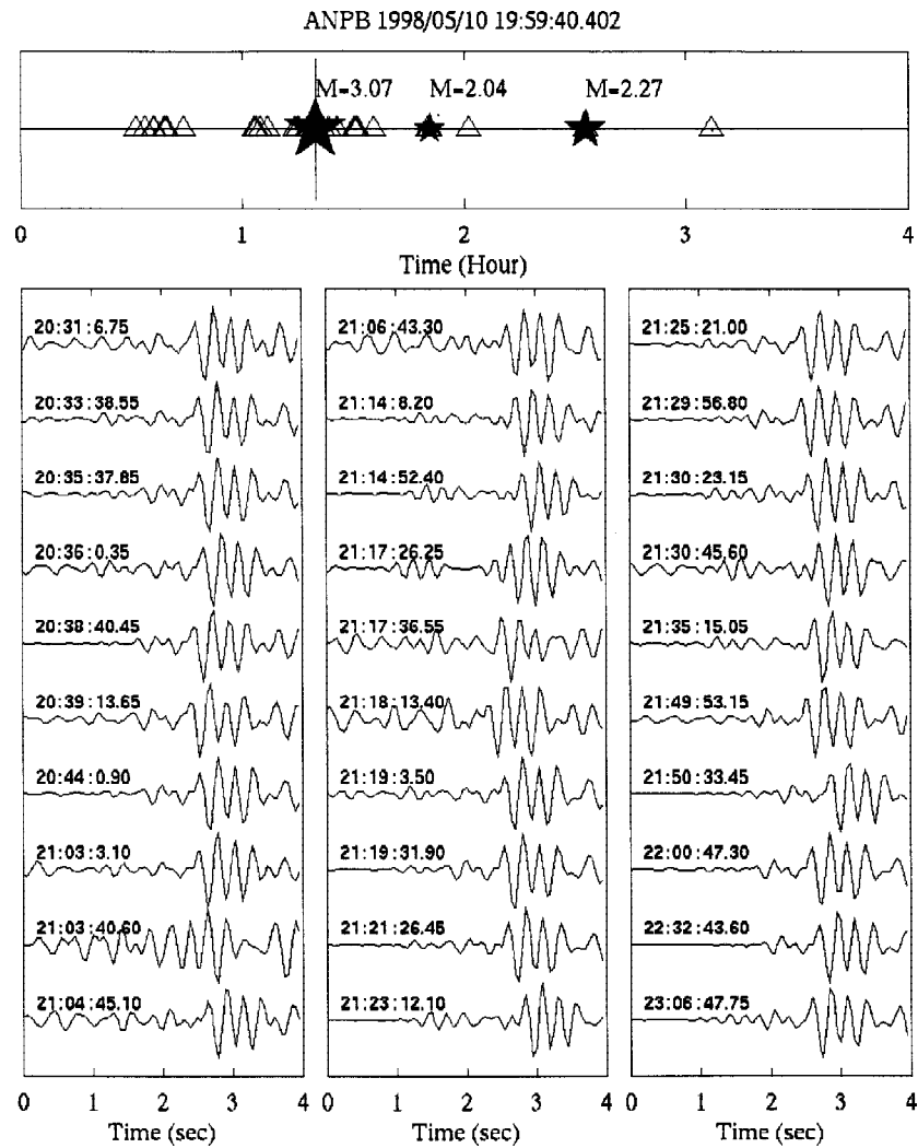
Fig. 6. Four hours time history of continuous data (vertical component) recorded at BATS-ANPB (upper panel) showing the occurrence of many microearthquakes not reported in the CWB catalog (open triangles) and three larger earthquakes (solid stars) that were reported in the CWB catalog. Examples of thirty bandpass filtered (4 - 10 Hz) vertical component seismograms for the newly identified earthquakes are shown in the lower panels. P-wave arrival time is shown in the upper-left corner of each trace.
