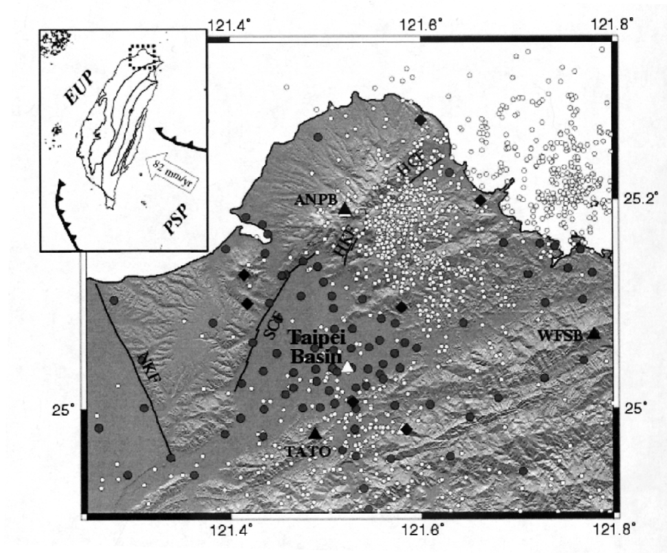
Fig. 1. Locations of seismic stations operated by various seismic networks and earthquake epicenters on top of topography map in the study area. The city of Taipei is located in the Taipei basin adjacent to the Tatun volcano group. Earthquake epicenters with magnitude greater than 2.0 between 1973 and 2003 are shown by open circles. Earthquake parameters are determined by TTSN-IES or TSN-CWB. Concentrated seismicity to the north and northeast of Taipei basin can be associated with the Tatun volcano group. TTSN-IES short period seismic stations, TSN-CWB short period seismic stations, TSMIP strong motion stations, and BATS broadband stations are shown as solid diamonds, open triangles, gray circles, and solid triangles, respectively. Locations of active fault (Lee 1999) are shown by solid lines including: HCF: Huangchi fault, HKF: Hsiaoyukeng fault, SCF: Sanchiao fault, and NKF: Nankan fault. The study area is marked by a rectangle with broken lines shown in the index map. The index map also shows NS-trending major geologic divisions in Taiwan. High convergence rate ( 82 \text{ mm yr}^{-1} ) and its direction are determined from GPS observations between 1990 and 1995 (Yu et al. 1997). EUP: Eurasian Plate, PSP: Philippine Sea Plate.
