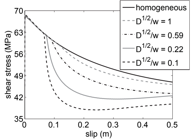
Figure 7. Plot of shear stress as a function of slip for varying diffusion constants scaled by the half-width of the fault gouge \sqrt{D}/w at a point on the fault 2 km from the hypocenter. In each case, the dynamically selected shear band width in the fault gouge is proportional to the effective temperature diffusion length scale. The uppermost curve is a “homogeneous” rupture for comparison, where the initial effective temperature is spatially uniform and no shear band forms. The other curves are all “localized” ruptures. The uppermost curve that includes diffusion ( \sqrt{D}/w = 1 ) is a “broad shear band,” as the diffusion length scale is equal to the gouge width. The lowermost curve is a “narrow shear band” with a diffusion length scale that is significantly smaller than the gouge half-width ( \sqrt{D}/w = 0.1 ). As the diffusion length scale decreases, the shear band becomes narrower, and the stress decreases more rapidly and reaches a lower value. The variation of stress as a function of slip with the diffusion length scale shows that strain localization is a mechanism for dynamic weakening.
