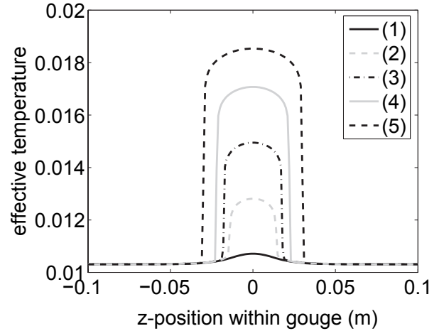
Figure 9. Plot of effective temperature as a function of z -position within the gouge at a point 2 km from the hypocenter at representative points shown in the stress versus slip plot (Figure 8). The horizontal range in this plot shows the entire gouge width in the simulation. The effective temperature is spatially uniform after 0.1 m of slip, at which point the feedbacks amplify the initial perturbation and a shear band forms. As slip propagates, the effective temperature increases and diffuses outwards. For slip beyond 0.3 m, the effective temperature decreases due to the relaxation term and maintains the width in curve (5). The diffusion constant in this simulation is \sqrt{D}/w = 0.2236 , and the initial stress is \tau_0 = 47 MPa.
